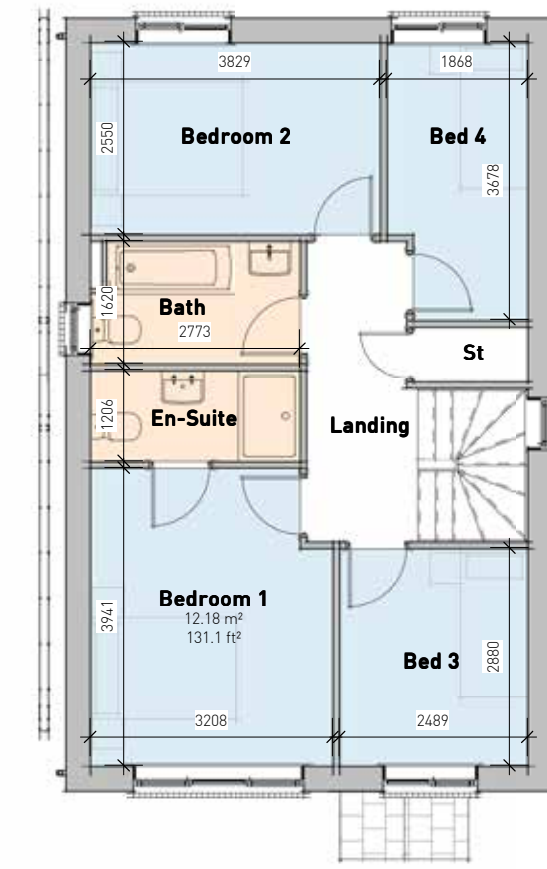
First Floor Plan - Ensuite
